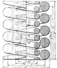
Fig. 1762. Helical Spring Class H24 for Atlantic (4-4-2) Locomotive. P. R. R.
